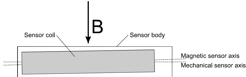
Fig. 9 Magnetic Misalignment
