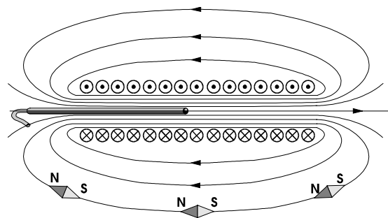
Fig 4: Measurement inside an Air Coil
