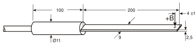
Transverse probe
