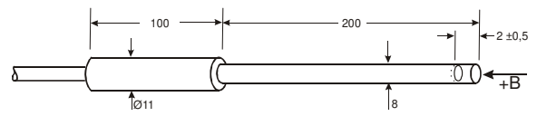
Axial probe
