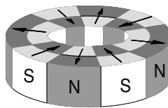
Figure 5 Magnetization radial
